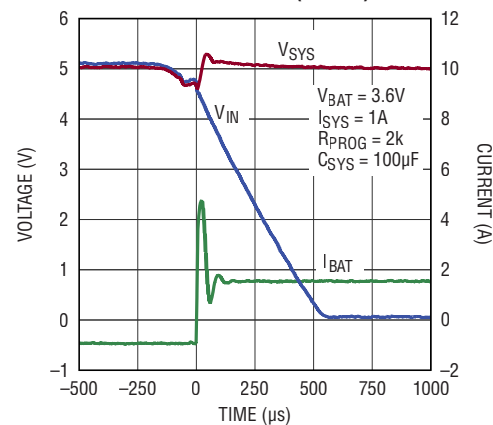
Normal to Backup Mode Transition Waveform (Li-Ion)
