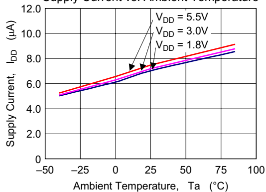
Figure 1-3 HA1631D01 Supply Current vs. Ambient Temperature
