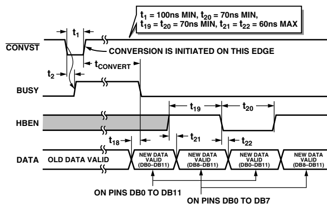
Figure 36. Read Cycle Timing Diagram with \overline{\text{CS}} and \overline{\text{RD}} Tied Low
