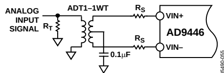
Figure 58. Transformer-Coupled Analog Input Circuit
