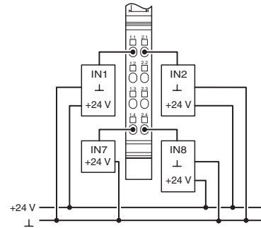
Figure 5 Example of a connection of sensors when using external busbars
