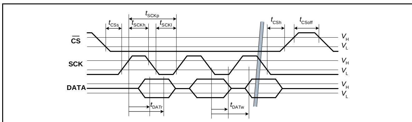
Figure 12 SSC Timing Definition
