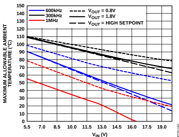
Figure 83. Ambient Temperature vs. V_{IN} for 10-Lead MSOP (171°C/W), 4-Layer EVB, C_{IN} = 4.3 \text{ nF} (Upper-/Lower-Side MOSFET)
