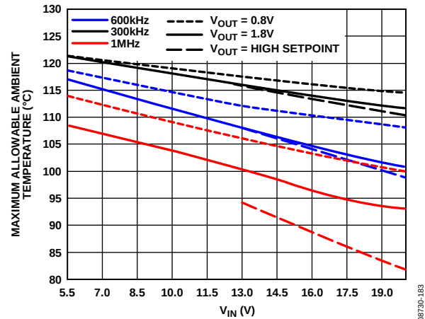
Figure 84. Ambient Temperature vs. V_{IN} for 10-Lead LFCSP (40°C/W), 4-Layer EVB, C_{IN} = 4.3 \text{ nF} (Upper-/Lower-Side MOSFET)
