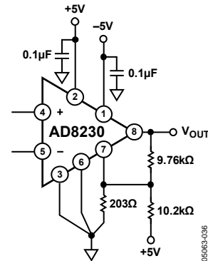
Figure 36. An AD8230 with its Output Biased at -4.8\text{ V} ; G = 100 ; V_{DESIRE\text{-}LEVEL} = -4.8\text{ V}
