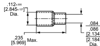
Ferrule Part No. 1-332057-0
