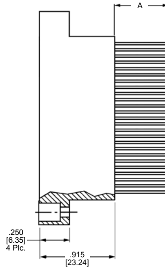
Receptacle Assembly
