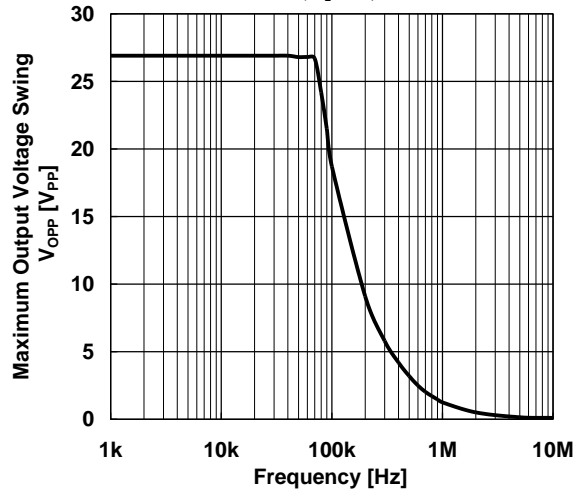
Maximum Output Voltage Swing vs. Frequency
