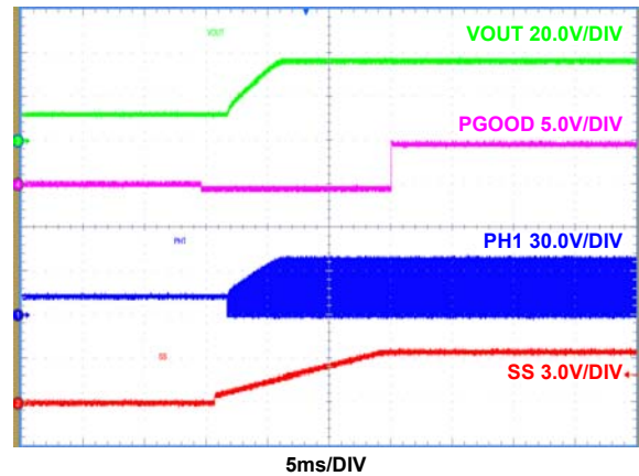
FIGURE 10. SOFT-START, DE+PHDRP MODE (DE/PHDRP = FLOAT), I_{OUT} = 8A
