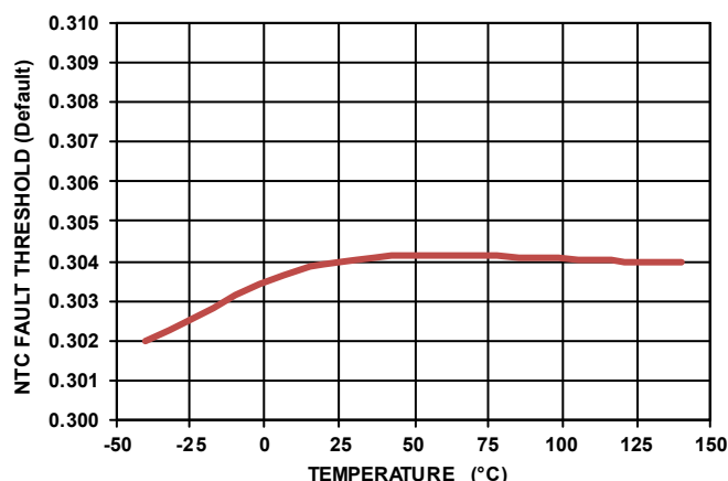
FIGURE 58. NTC FAULT THRESHOLD (DEFAULT) vs TEMPERATURE
