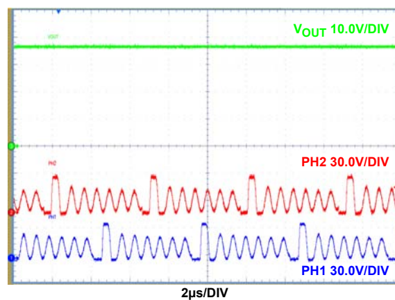
FIGURE 18. DE MODE (DE/PHDRP = V_{CC} ), DIODE EMULATION OPERATION, I_{OUT} = 29mA
