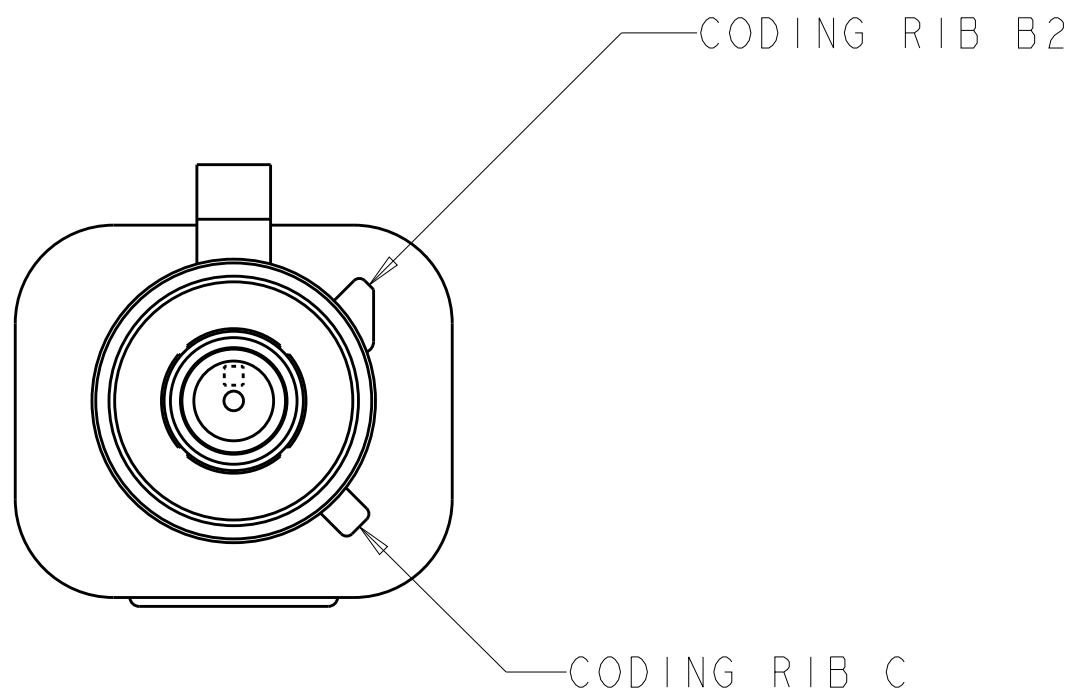
DETAIL H
