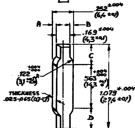
PANEL CUT-OUT
