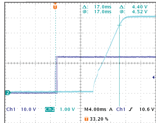
On/Off Enable Startup (V IN =24V, V OUT =5V, I OUT =3A, C LOAD =0)
