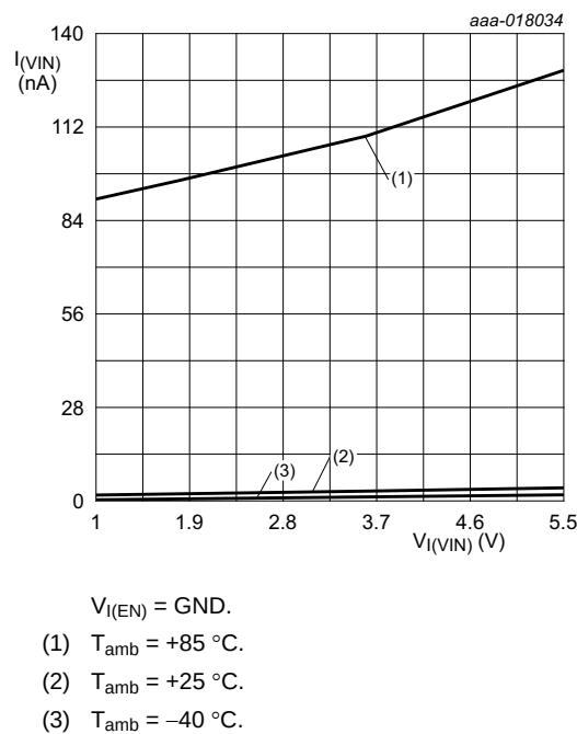
Fig 9. Typical supply current versus input voltage on pin VIN
