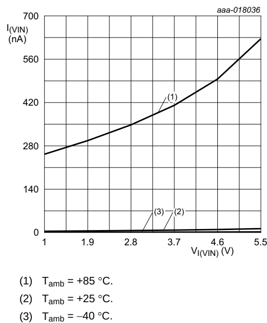
Fig 11. Typical OFF-state leakage current versus input voltage on pin VIN
