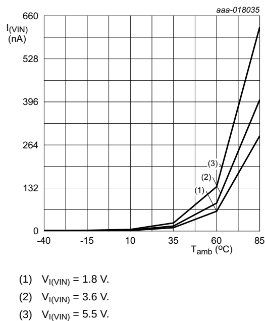
Fig 10. Typical OFF-state leakage current versus temperature
