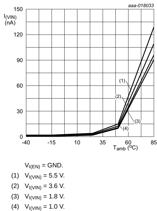
Fig 8. Typical supply current versus temperature
