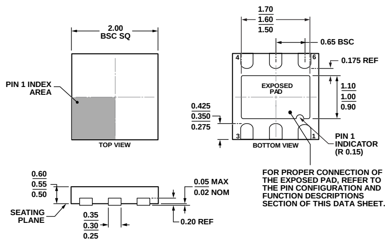
Figure 55. 6-Lead Lead Frame Chip Scale Package [LFCSP_UD] 2.00 mm × 2.00 mm Body, Ultra Thin, Dual Lead (CP-6-3)
