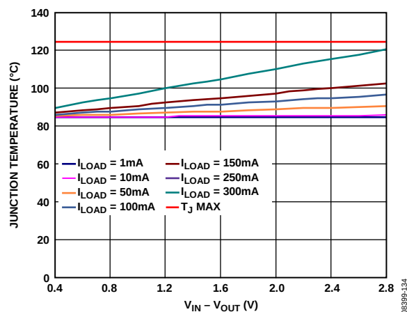
Figure 44. Junction Temperature vs. Power Dissipation, Board Temperature = 85^\circ\text{C}
