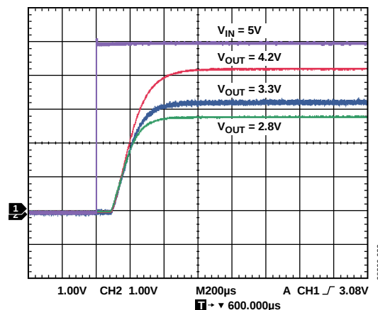
Figure 37. Typical Start-Up Time
