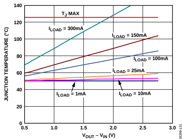
Figure 41. Junction Temperature vs. Power Dissipation, 500 \text{mm}^2 of PCB Copper, T_A = 50^{\circ}\text{C}
