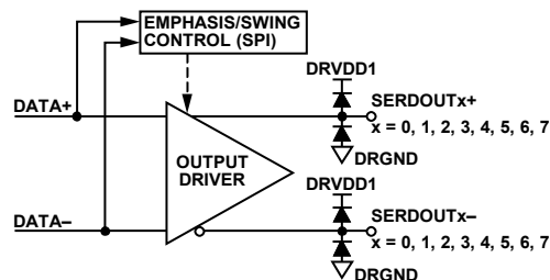
Figure 70. Digital Outputs
