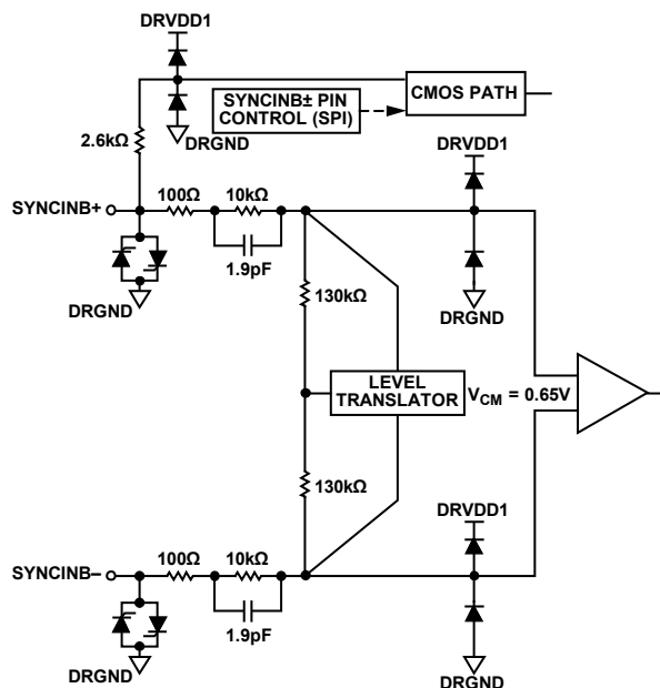
Figure 68. SYNCINB± Inputs
