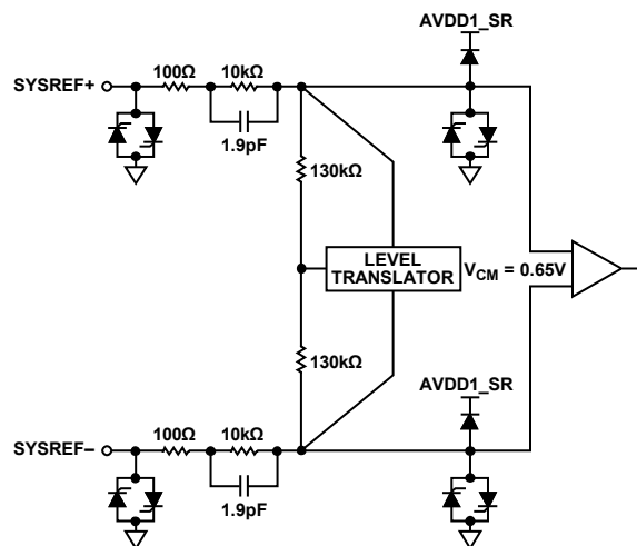
Figure 69. SYSREF± Inputs
