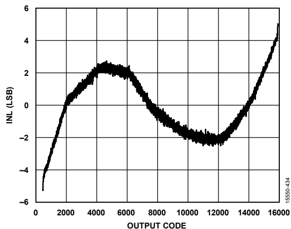
Figure 34. INL, f_{IN} = 155 MHz
