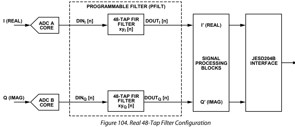
Figure 104. Real 48-Tap Filter Configuration
