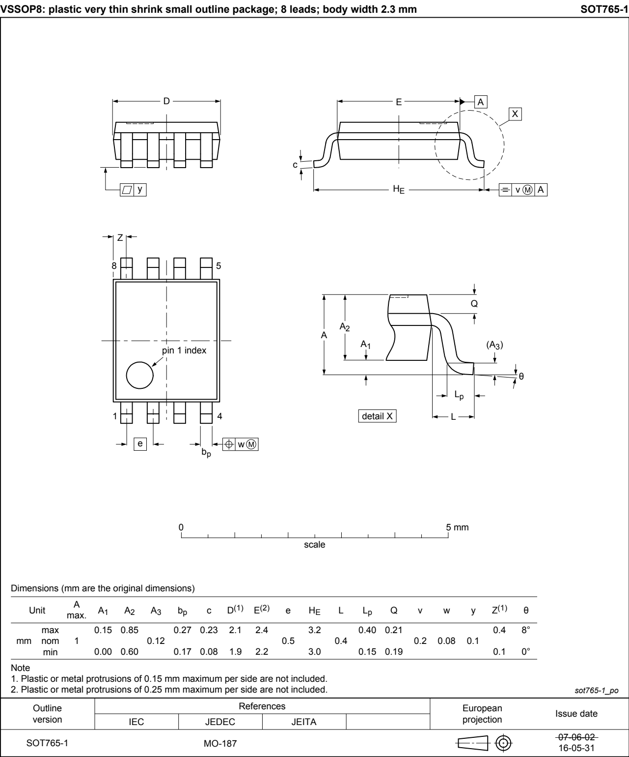
Figure 11. Package outline SOT765-1 (VSSOP8)
