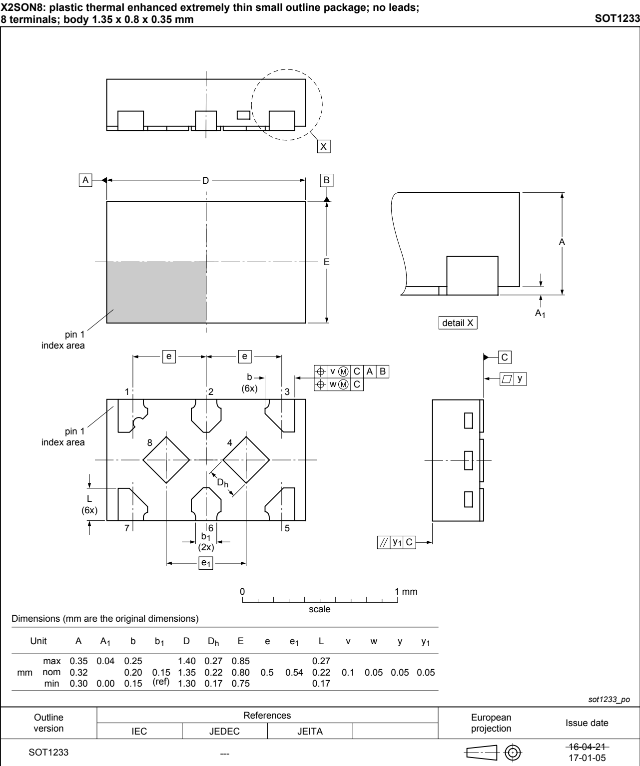
Figure 17. Package outline SOT1233 (X2SON8)
