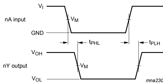
Figure 8. The data input (nA) to output (nY) propagation delays
