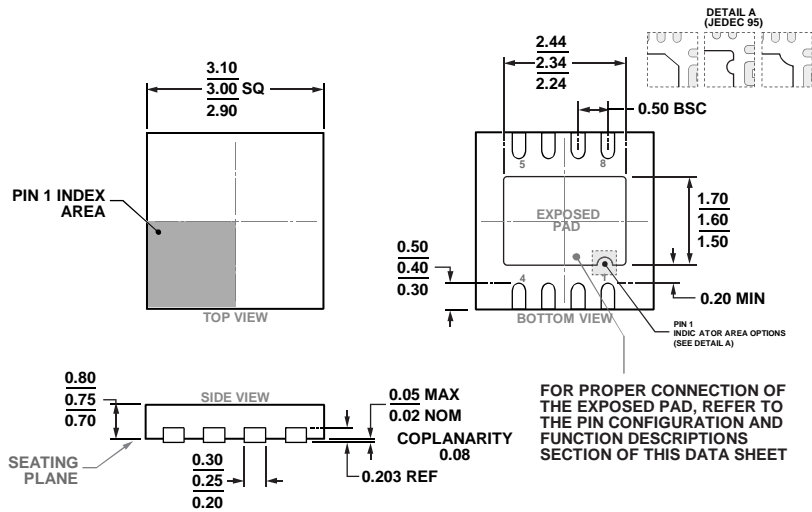
COMPLIANT TO JEDEC STANDARDS MO-229-W3030D-4 Figure 80. 8-Lead Lead Frame Chip Scale Package [LFCSP] 3 mm x 3 mm Body and 0.75 mm Package Height (CP-8-11) Dimensions shown in millimeters
