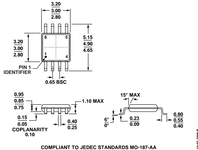
Figure 79. 8-Lead Mini Small Outline Package [MSOP] (RM-8) Dimensions shown in millimeters
