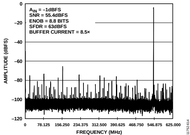
Figure 14. Single-Tone FFT with f_{IN} = 1954.3 MHz
