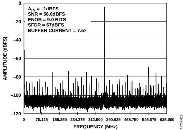
Figure 13. Single-Tone FFT with f_{IN} = 1602.3 MHz
