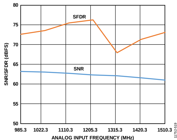
Figure 67. SNR/SFDR vs. f_{IN} ; 1 \text{ GHz} < f_{IN} < 1.5 \text{ GHz} ; Buffer Control 1 (0x018) = 6.5x
