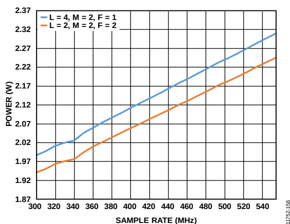
Figure 103. Power Dissipation vs. f_s
