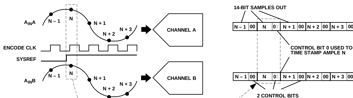
Figure 174. AD9680 Timestamping—CS = 2 (Register 0x58F, Bits[7:6] = 2), Control Bit 1 is SYSREF± (Register 0x559, Bits[6:4] = 5)
