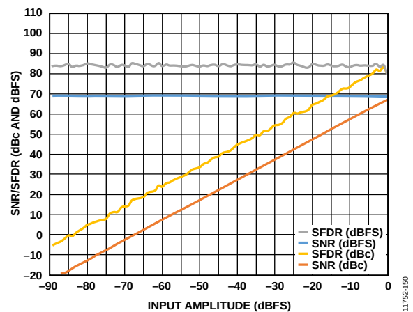
Figure 97. SNR/SFDR vs. Analog Input Level, f_{IN} = 170.3\text{ MHz}
