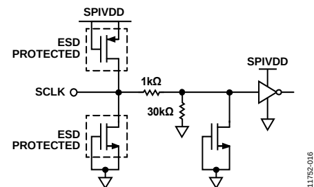
Figure 109. SCLK Input
