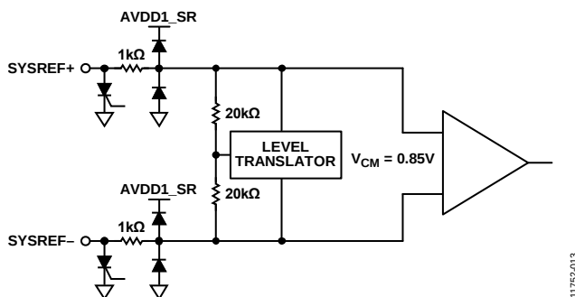
Figure 106. SYSREF± Inputs
