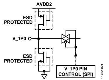
Figure 114. V_1P0 Input/Output
