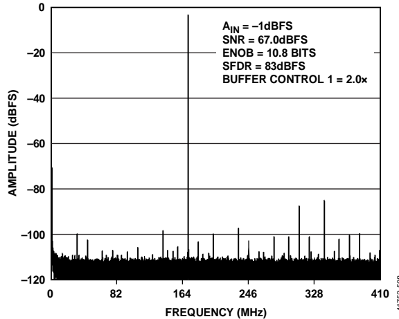
Figure 56. Single-Tone FFT with f_{IN} = 170.3 MHz
