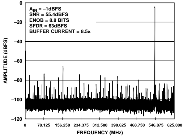
Figure 14. Single-Tone FFT with f_{IN} = 1954.3 \text{ MHz}
