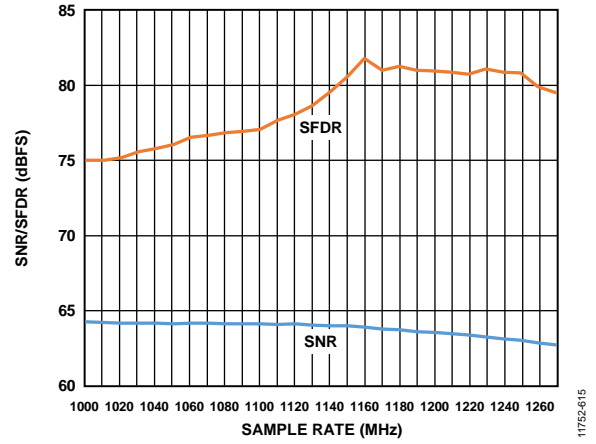
Figure 15. SNR/SFDR vs. f_s , f_{IN} = 170.3 \text{ MHz} ; Buffer Control 1 (0x018) = 3.5x
