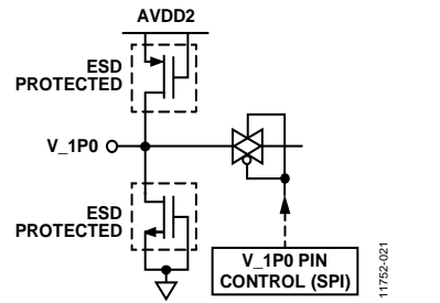
Figure 114. V_1P0 Input/Output
