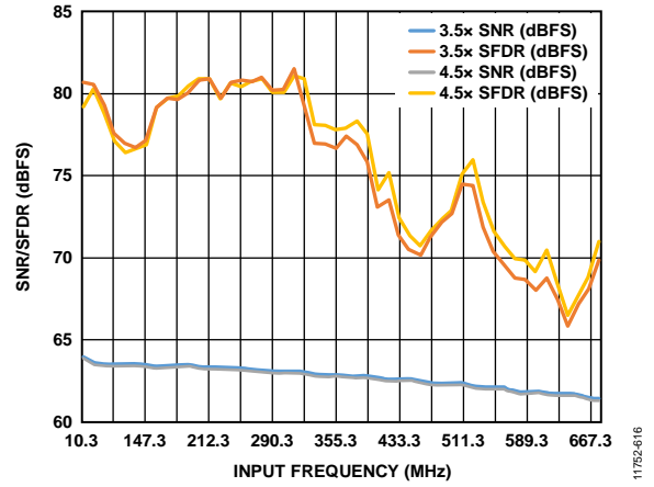
Figure 16. SNR/SFDR vs. f_{IN} ; f_{IN} < 700 \text{ MHz} ; Buffer Control 1 (0x018) = 3.5x and 4.5x
