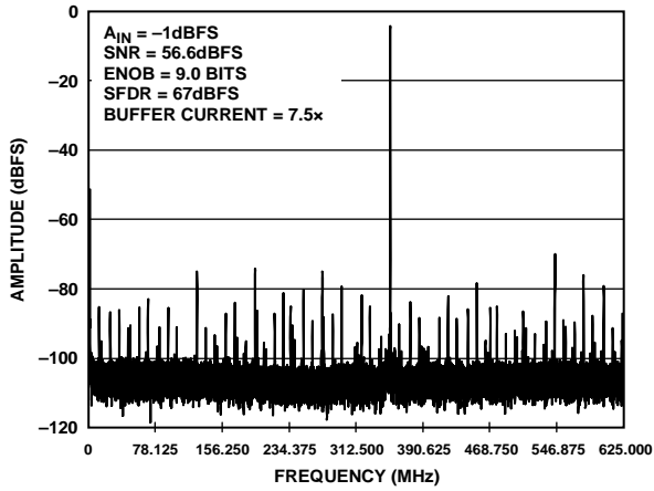
Figure 13. Single-Tone FFT with f_{IN} = 1602.3 \text{ MHz}
