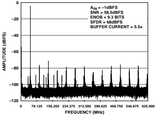
Figure 12. Single-Tone FFT with f_{IN} = 1205.3 \text{ MHz}
