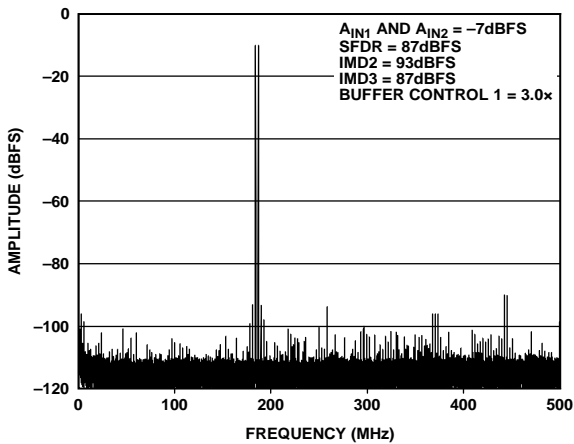
Figure 44. Two-Tone FFT; f_{IN1} = 184\text{ MHz} , f_{IN2} = 187\text{ MHz}
