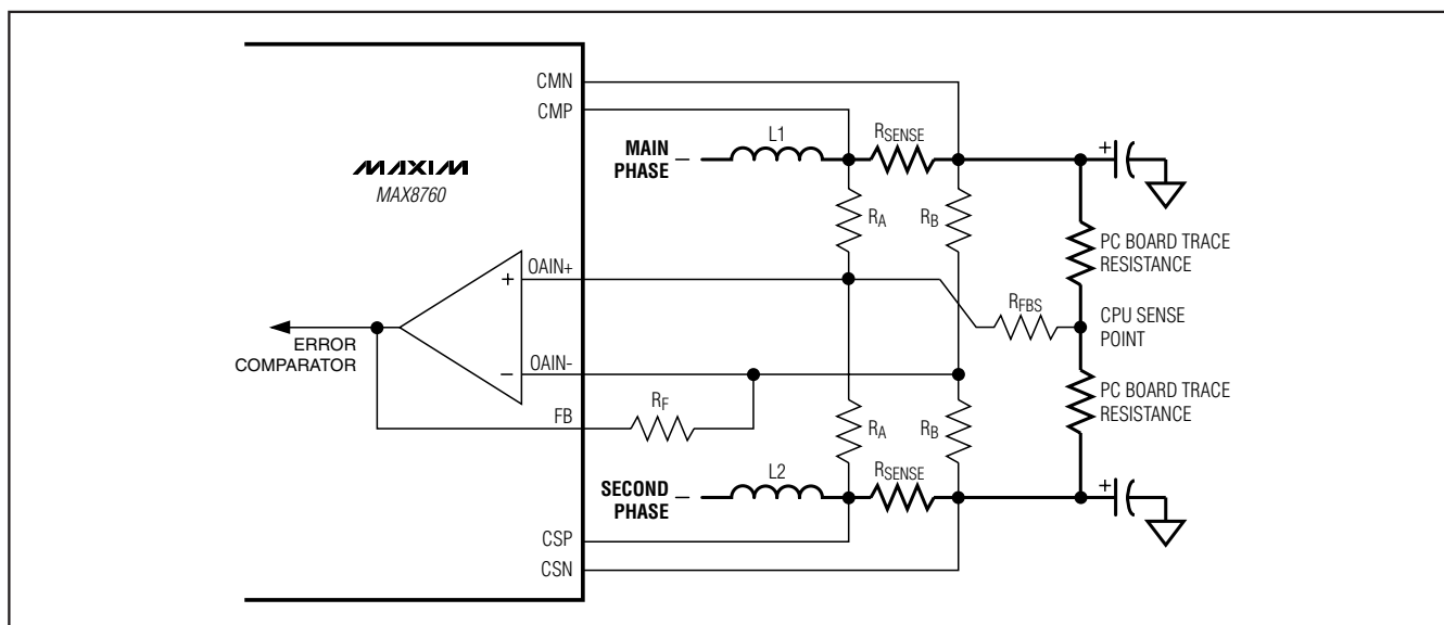
Figure 10. Voltage-Positioning Gain
