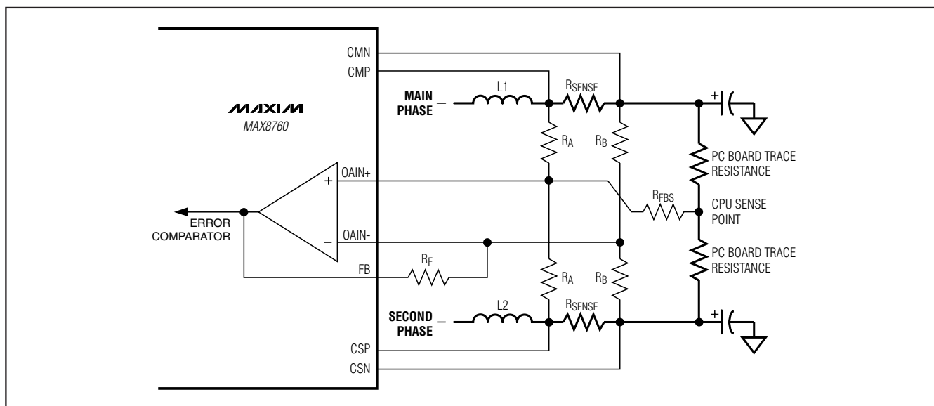
Figure 10. Voltage-Positioning Gain
