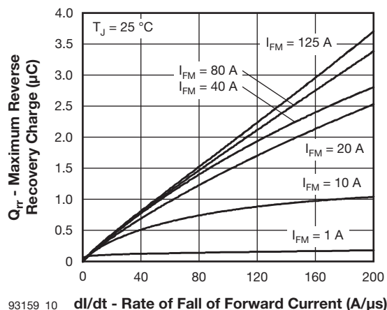
dl/dt - Rate of Fall of Forward Current (A/µs) Fig. 10 - Recovery Charge Characteristics, T_J = 25\text{ }^{\circ}\text{C}
