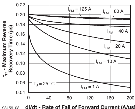
dl/dt - Rate of Fall of Forward Current (A/µs) Fig. 8 - Recovery Time Characteristics, T_J = 25\text{ }^{\circ}\text{C}
