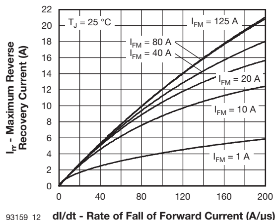
dl/dt - Rate of Fall of Forward Current (A/µs) Fig. 12 - Recovery Current Characteristics, T_J = 25\text{ }^{\circ}\text{C}
