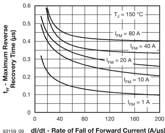
dl/dt - Rate of Fall of Forward Current (A/µs) Fig. 9 - Recovery Time Characteristics, T_J = 150\text{ }^{\circ}\text{C}
