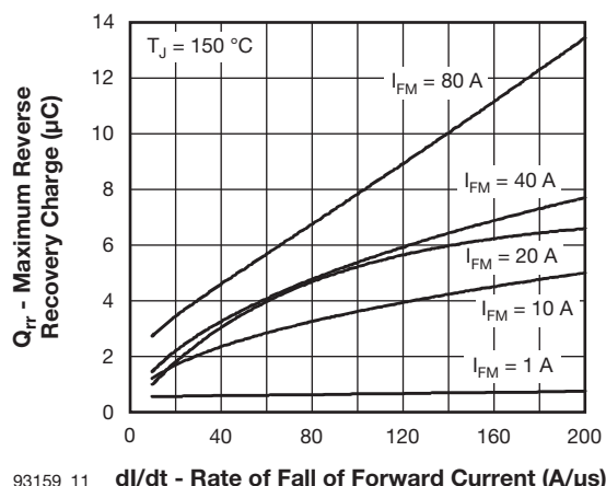
dl/dt - Rate of Fall of Forward Current (A/µs) Fig. 11 - Recovery Charge Characteristics, T_J = 150\text{ }^{\circ}\text{C}
