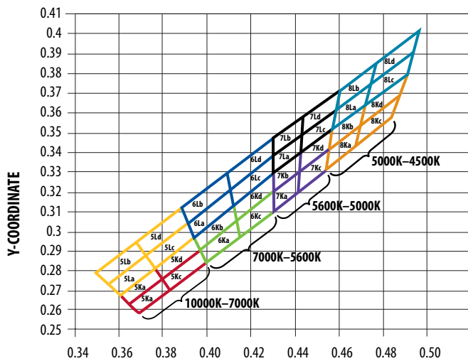
Color Bin Selection ( X_s ) for ASMT-QYBx
