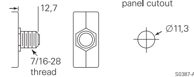
Mounting bushing
