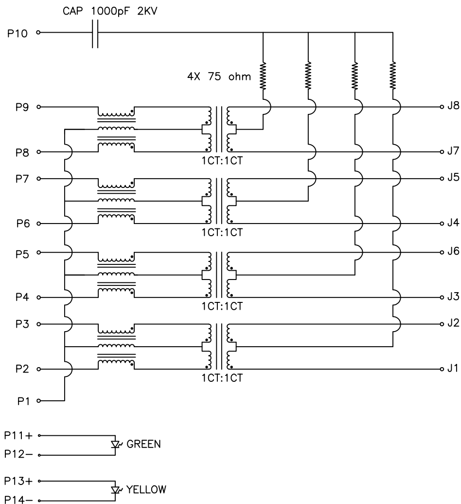
SCHEMATIC
