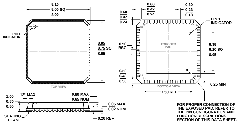
COMPLIANT TO JEDEC STANDARDS MO-220-VMM4-4 Figure 60. 64-Lead Lead Frame Chip Scale Package [LFCSP_VQ] 9 mm x 9 mm Body, Very Thin Quad (CP-64-4) Dimensions shown in millimeters
