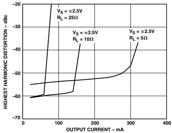
TPC 10. Distortion vs. Output Current; V_S = \pm 2.5V , f = 1\text{ MHz} , G = +2
