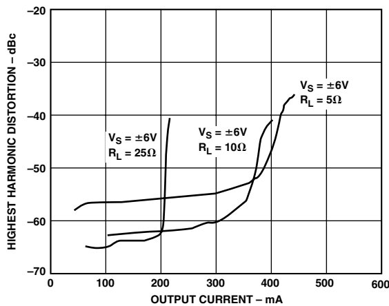
TPC 7. Distortion vs. Output Current; V_S = \pm 6V , f = 1\text{ MHz} , G = +2
