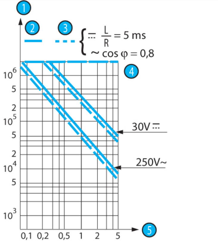
Operating curve for type 83229
