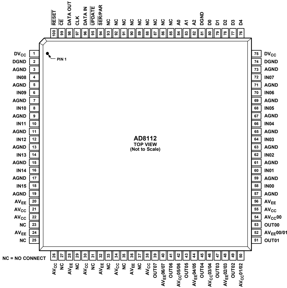
Figure 6. Pin Configuration
