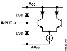
Figure 7. Analog Input
