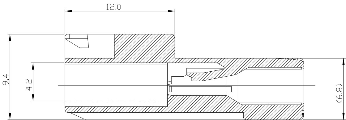
SECTION X-X
