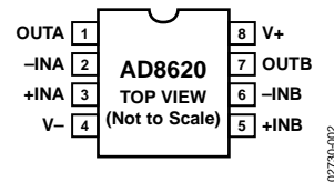
Figure 2. 8-Lead SOIC_N
