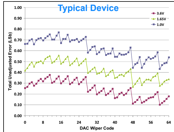
FIGURE 2-76: Total Unadjusted Error vs. Code and V_{REF} V_{DD} = 3.6\text{V} , V_{REF} = 1\text{V} , 1.65\text{V} , and 3.6\text{V} , Temp = +25^\circ\text{C} .
