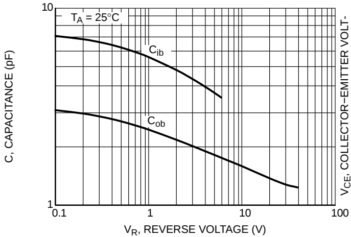
Figure 20. Capacitances
