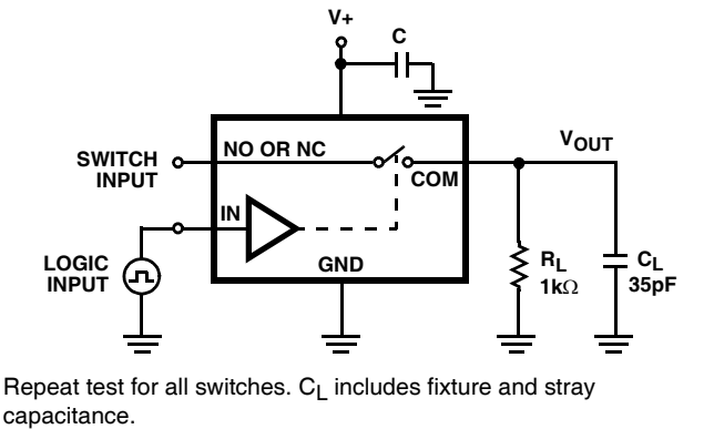
FIGURE 1B. TEST CIRCUIT
