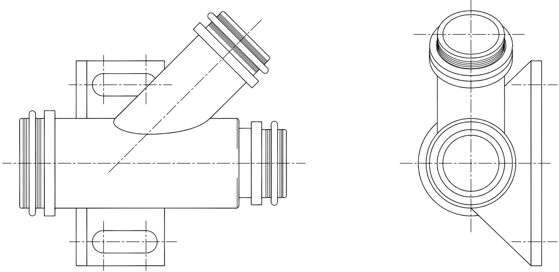
TRANSITION ASSEMBLY - 45°
